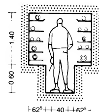
⑤ Section of main service route (walk-in) varies according to number of ducts it is carrying
